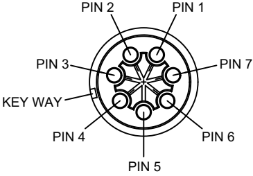
7 PIN FEMALE MATING FACE
