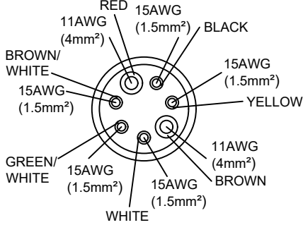
CABLE BUILDUP
